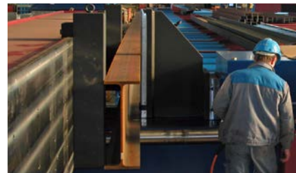
107 Beam straightening or bending in upright position
