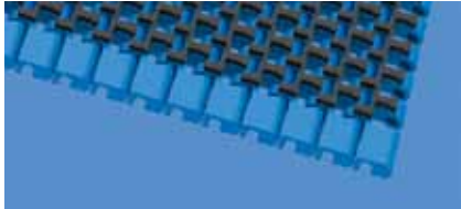
S14 | 25% open | Friction Top 1
