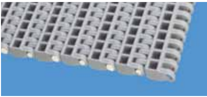
S8 | 25% open | Radius Top
