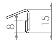
DETAIL C
